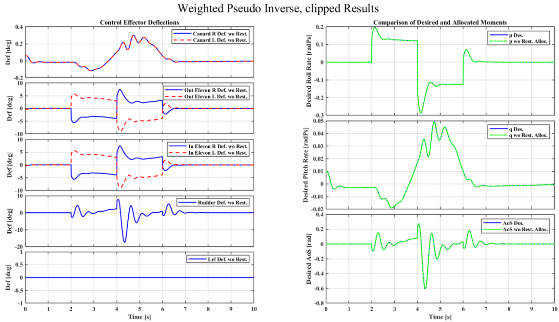
Figure 21: Scenario 1: Closed-Loop Results for Weighted Pseudo-Inverse (Clipped) Approach.
